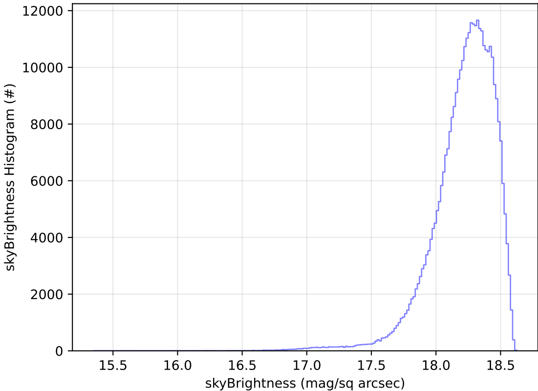
telescope_jerk_v3.5_10yrs WFD y band: skyBrightness Histogram
