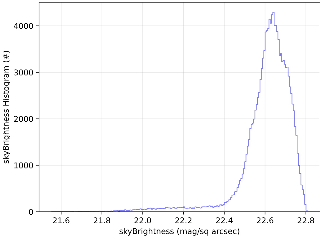
telescope_jerk_v3.5_10yrs WFD u band: skyBrightness Histogram
