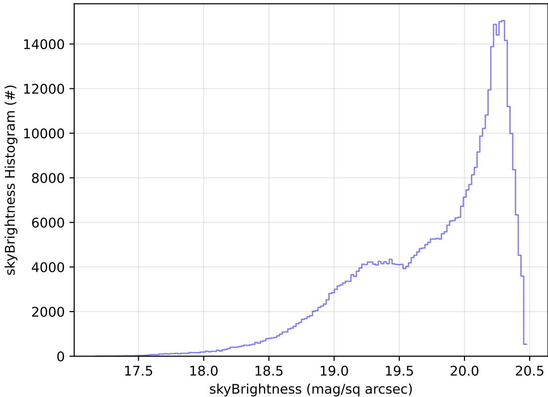
telescope_jerk_v3.5_10yrs WFD i band: skyBrightness Histogram
