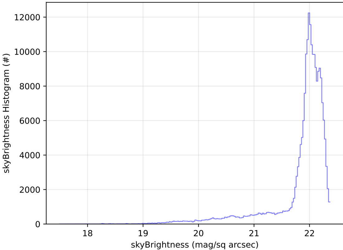
telescope_jerk_v3.5_10yrs WFD g band: skyBrightness Histogram
