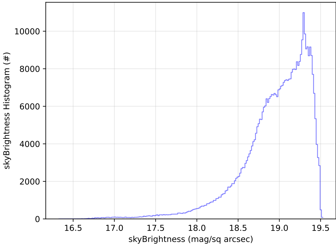
telescope_jerk_v3.5_10yrs All sky z band: skyBrightness Histogram
