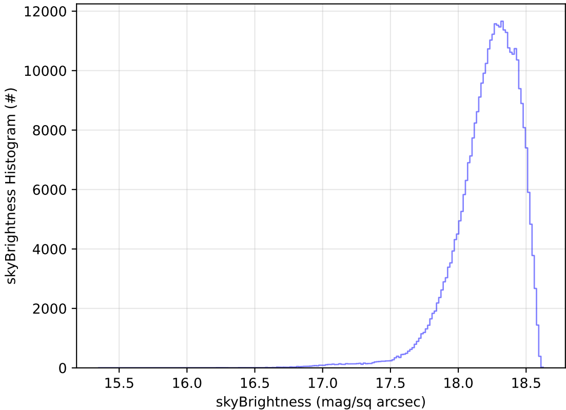
telescope_jerk_v3.5_10yrs All sky y band: skyBrightness Histogram
