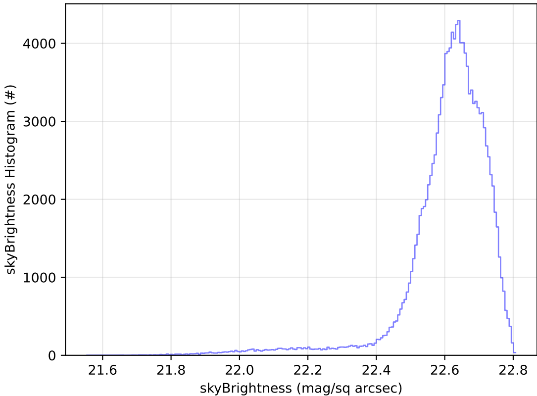
telescope_jerk_v3.5_10yrs All sky u band: skyBrightness Histogram
