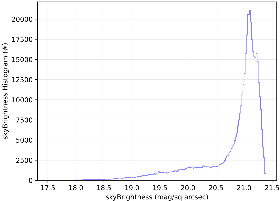
telescope_jerk_v3.5_10yrs All sky r band: skyBrightness Histogram
