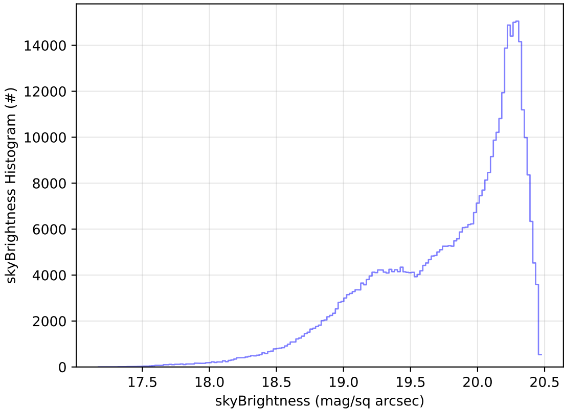
telescope_jerk_v3.5_10yrs All sky i band: skyBrightness Histogram
