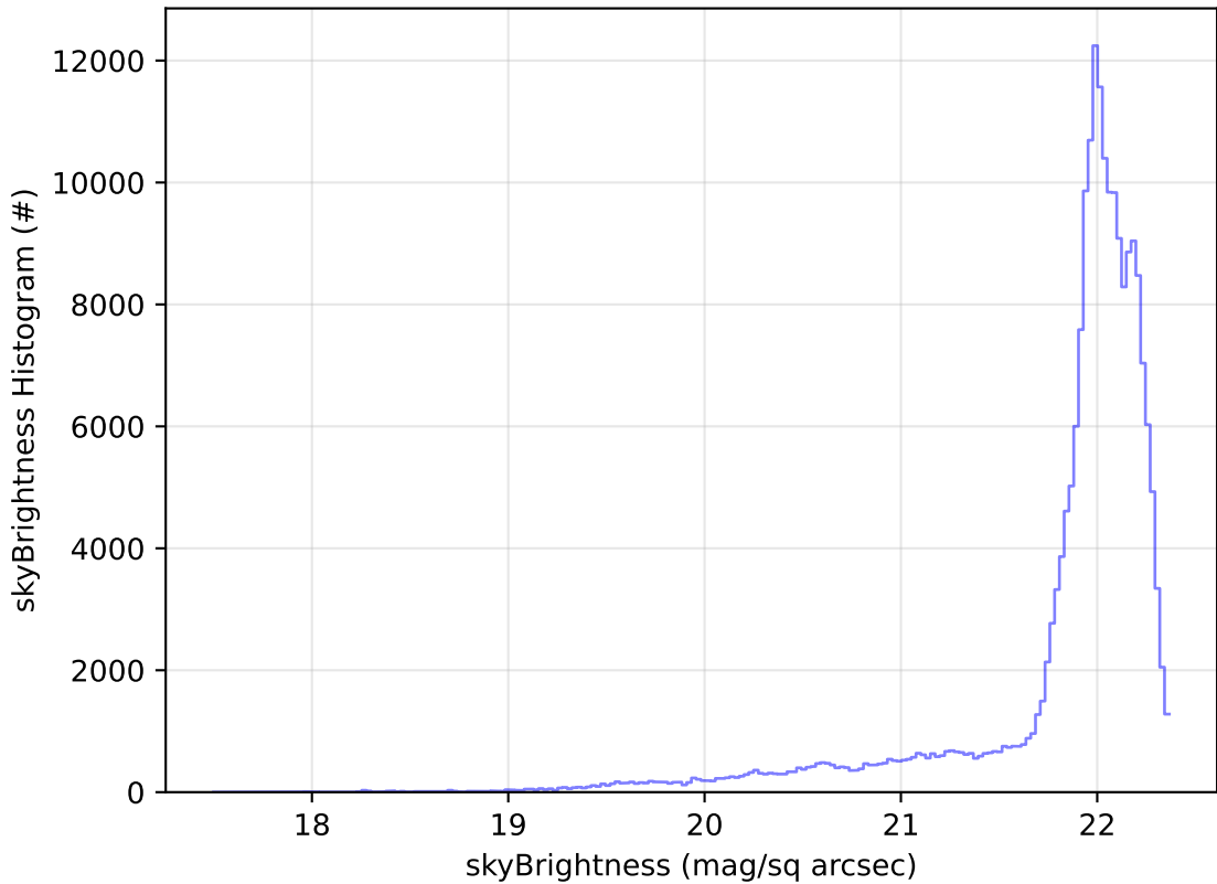
telescope_jerk_v3.5_10yrs All sky g band: skyBrightness Histogram
