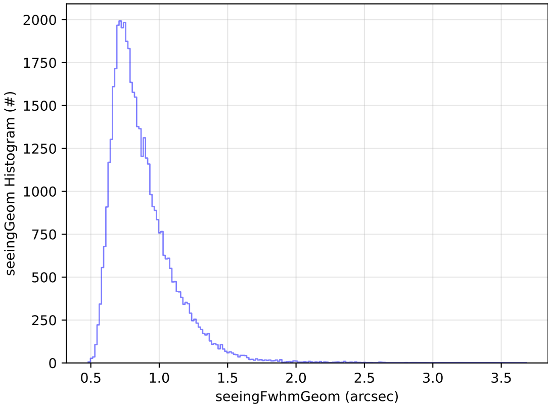
telescope_jerk_v3.5_10yrs Yr 1 z band: seeingGeom Histogram
