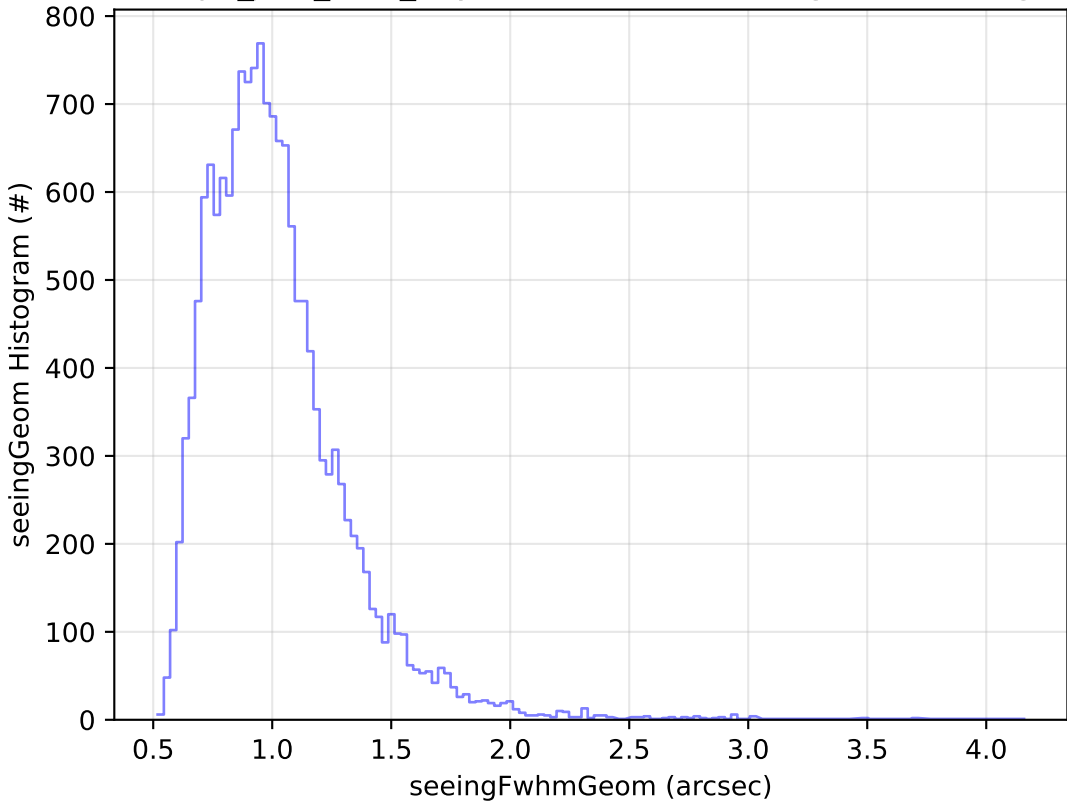
telescope_jerk_v3.5_10yrs Yr 1 u band: seeingGeom Histogram
