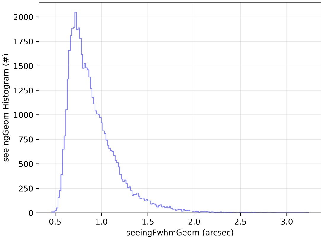
telescope_jerk_v3.5_10yrs Yr 1 r band: seeingGeom Histogram
