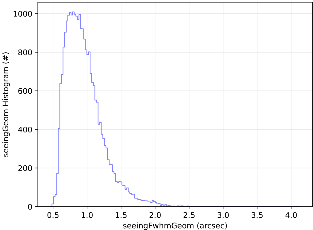
telescope_jerk_v3.5_10yrs Yr 1 g band: seeingGeom Histogram
