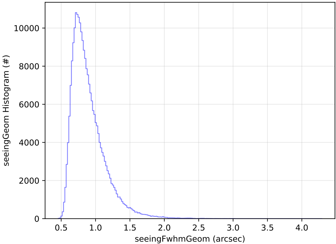
telescope_jerk_v3.5_10yrs Yr 1 all bands: seeingGeom Histogram
