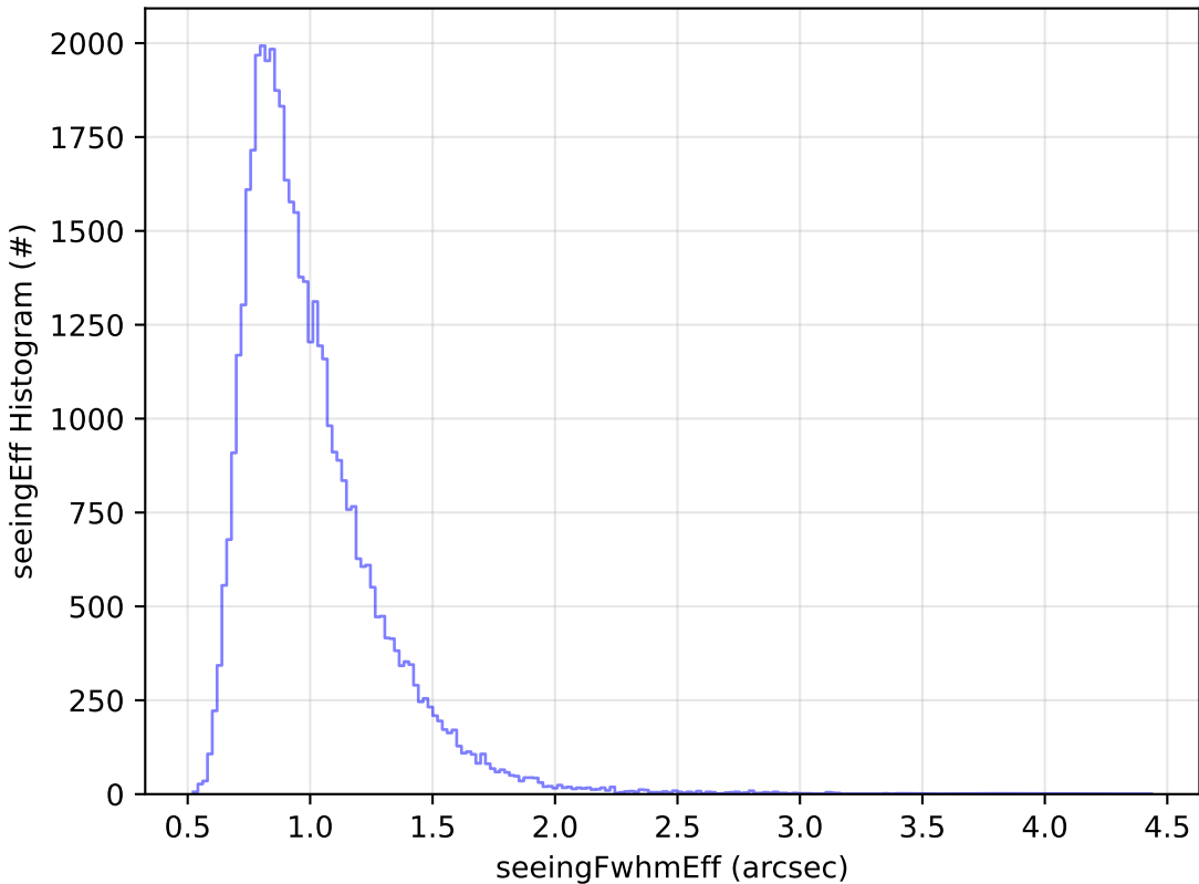
telescope_jerk_v3.5_10yrs Yr 1 z band: seeingEff Histogram
