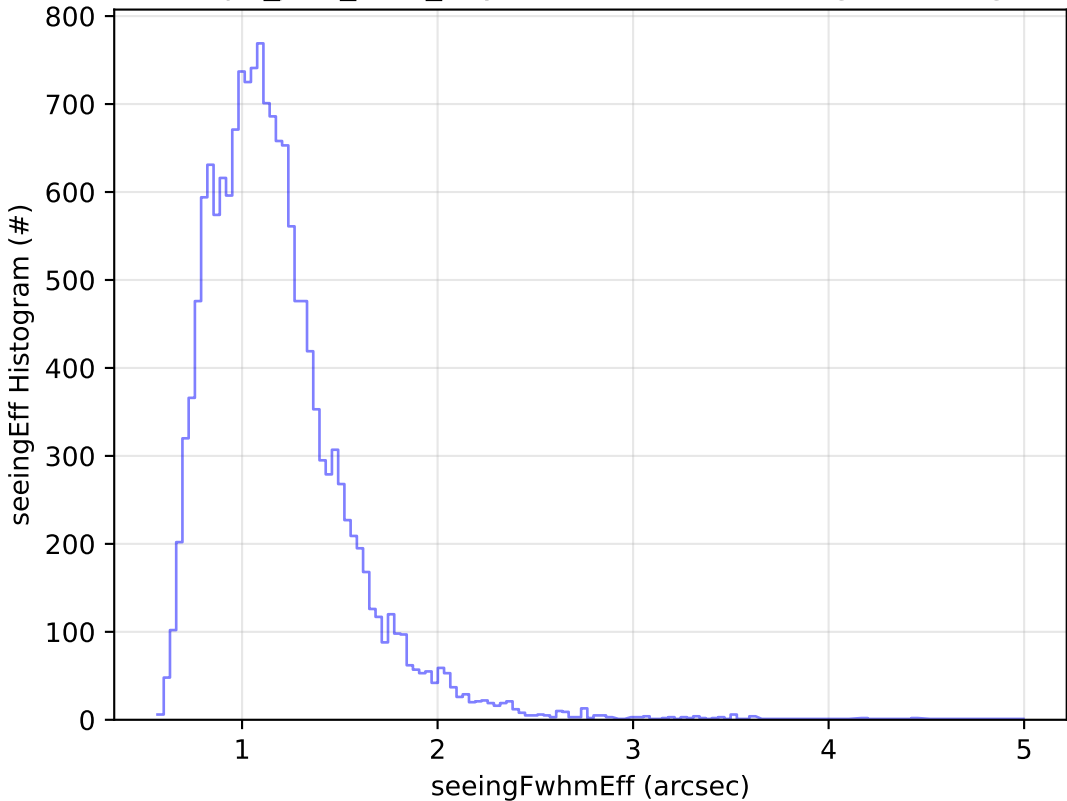
telescope_jerk_v3.5_10yrs Yr 1 u band: seeingEff Histogram
