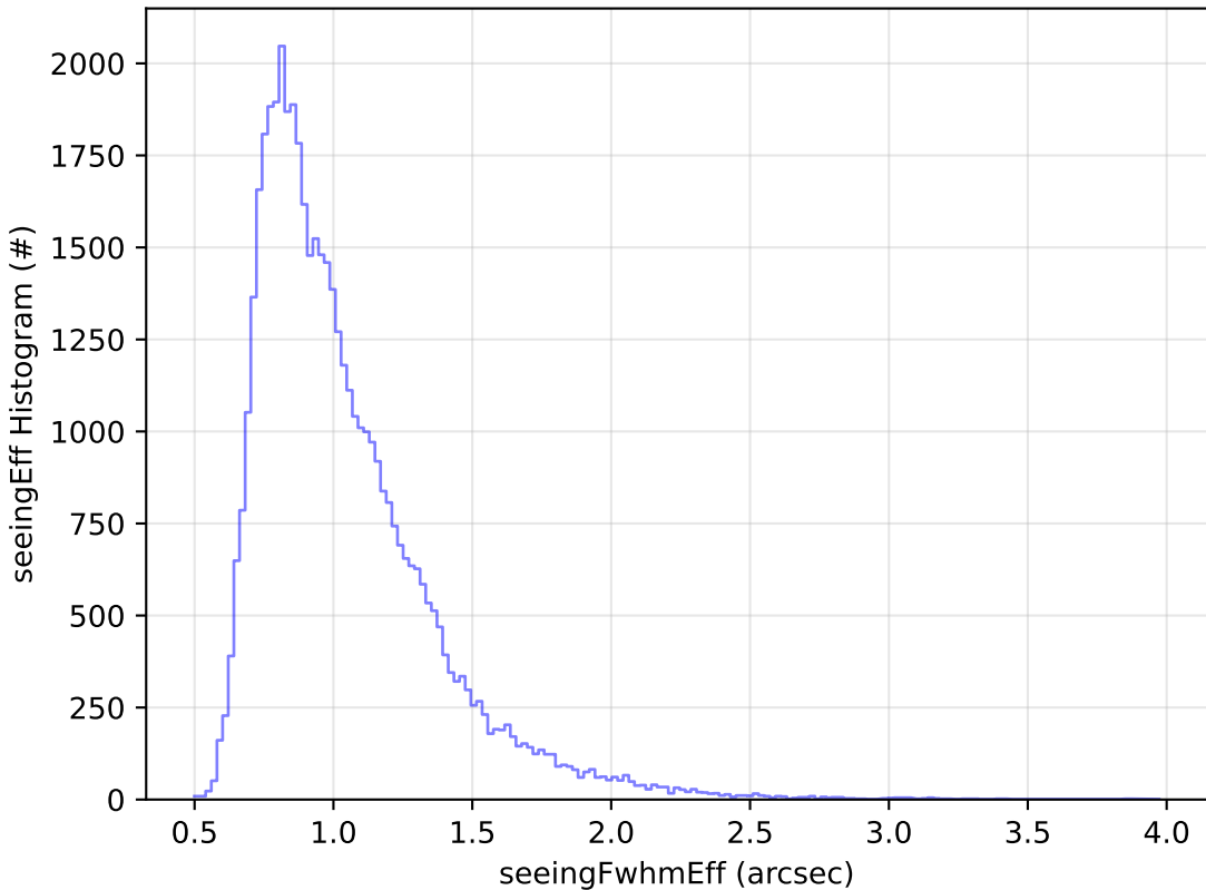
telescope_jerk_v3.5_10yrs Yr 1 r band: seeingEff Histogram
