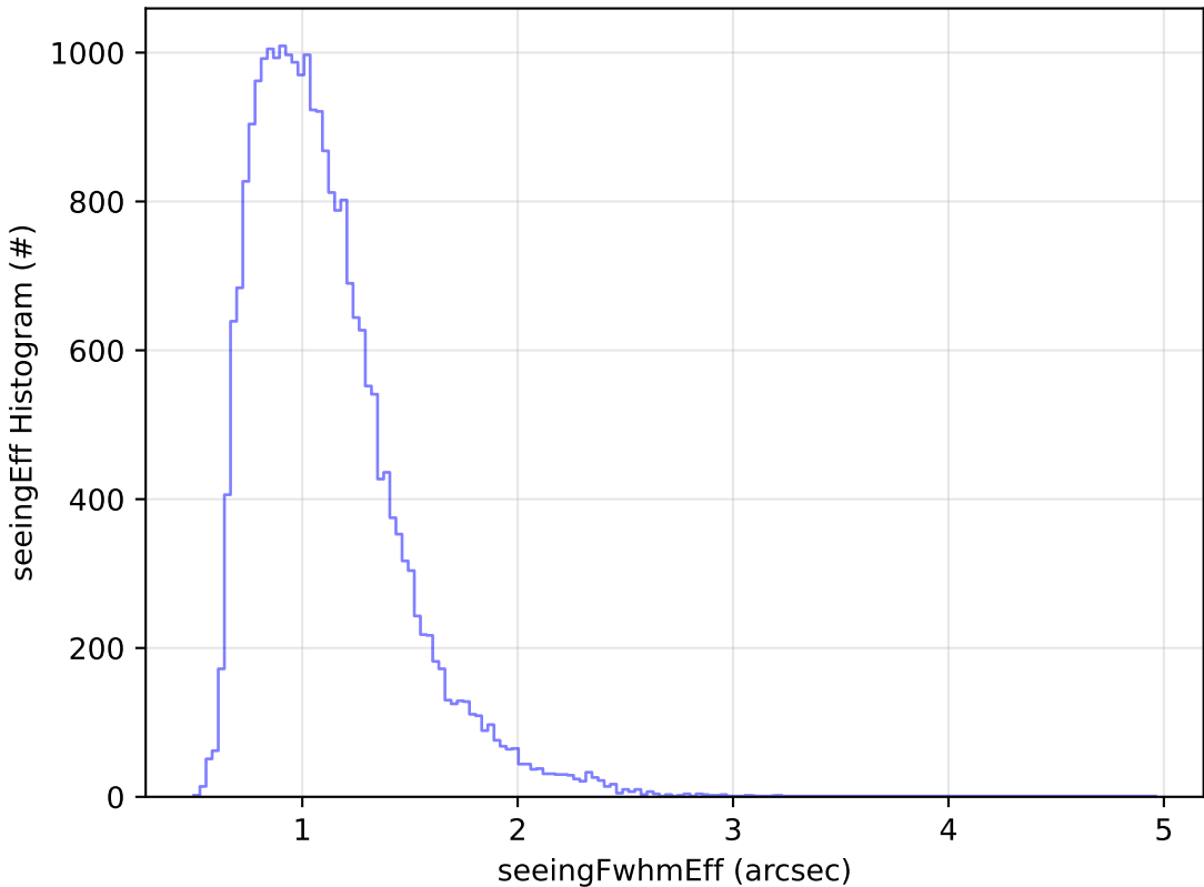
telescope_jerk_v3.5_10yrs Yr 1 g band: seeingEff Histogram
