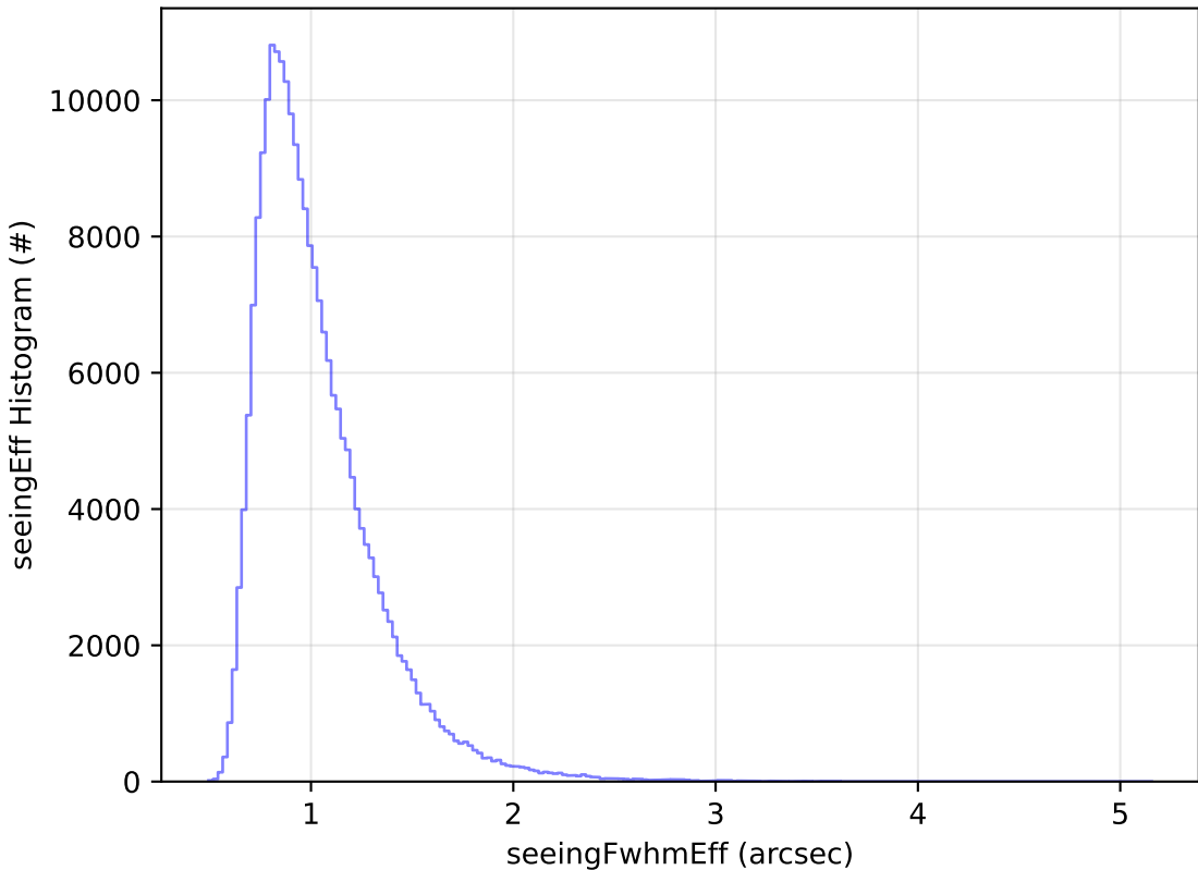
telescope_jerk_v3.5_10yrs Yr 1 all bands: seeingEff Histogram
