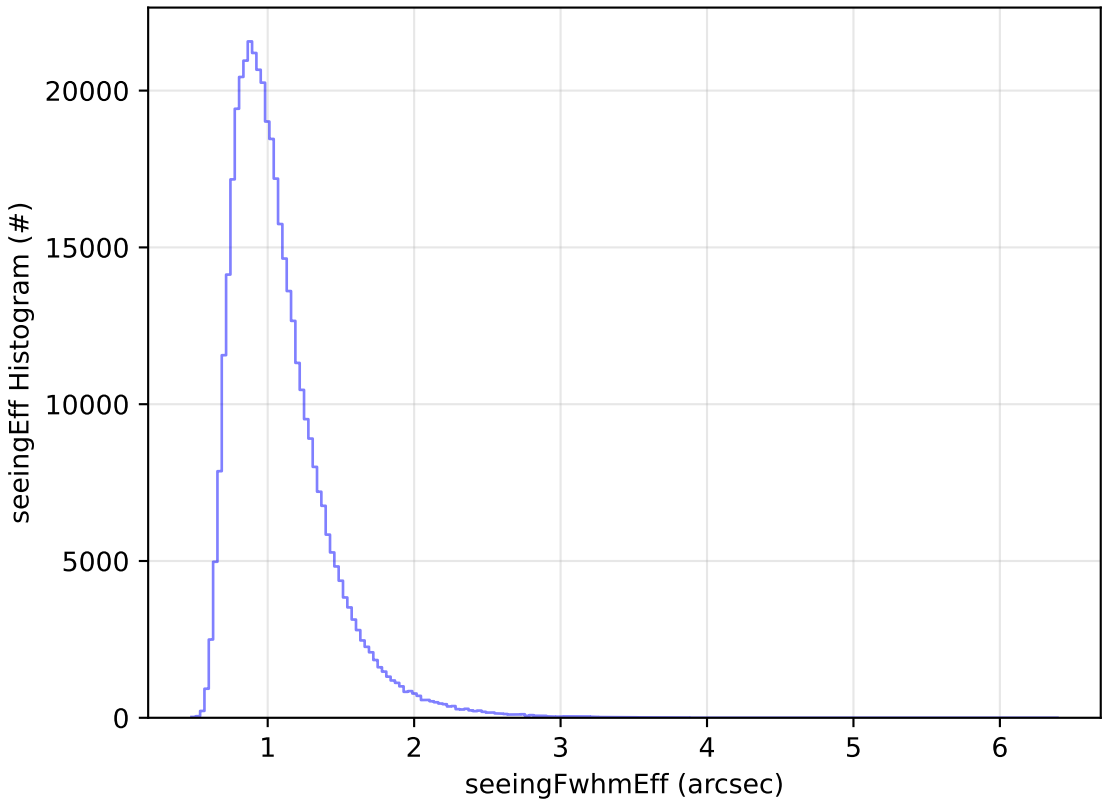
telescope_jerk_v3.5_10yrs WFD z band: seeingEff Histogram
