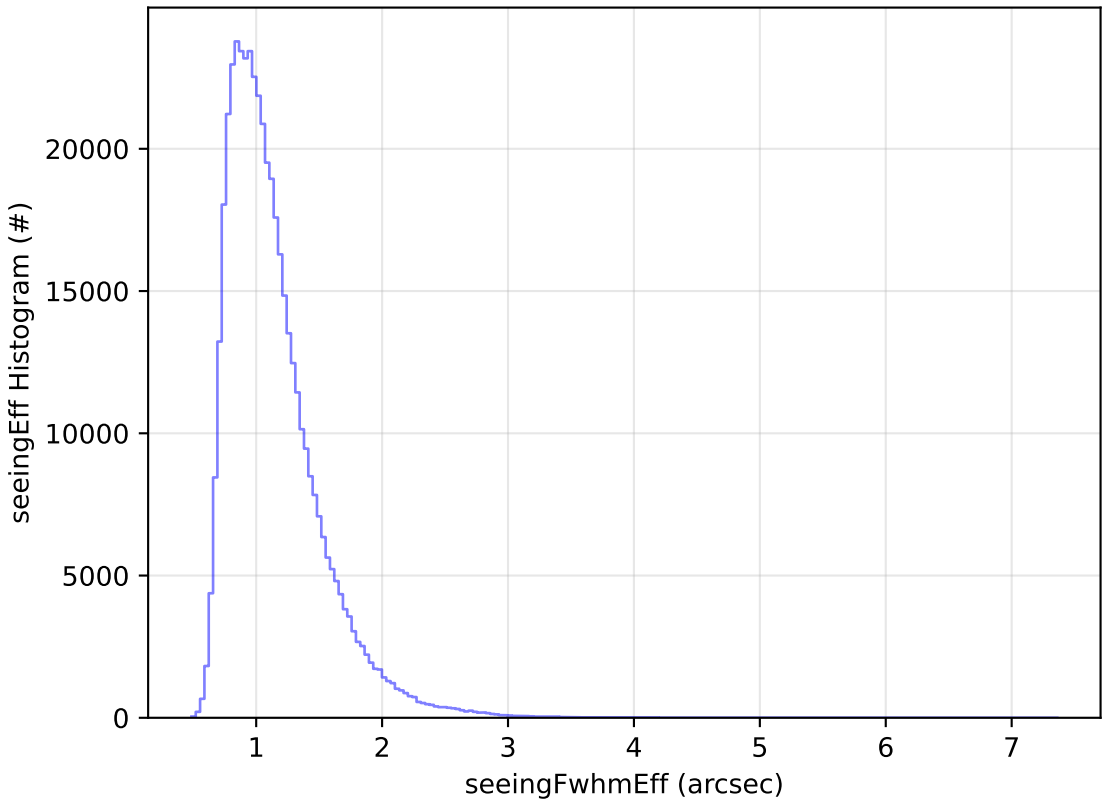
telescope_jerk_v3.5_10yrs WFD r band: seeingEff Histogram
