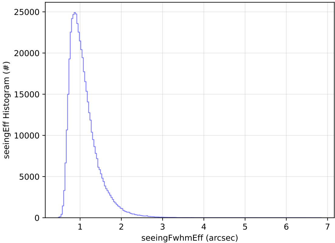
telescope_jerk_v3.5_10yrs WFD i band: seeingEff Histogram
