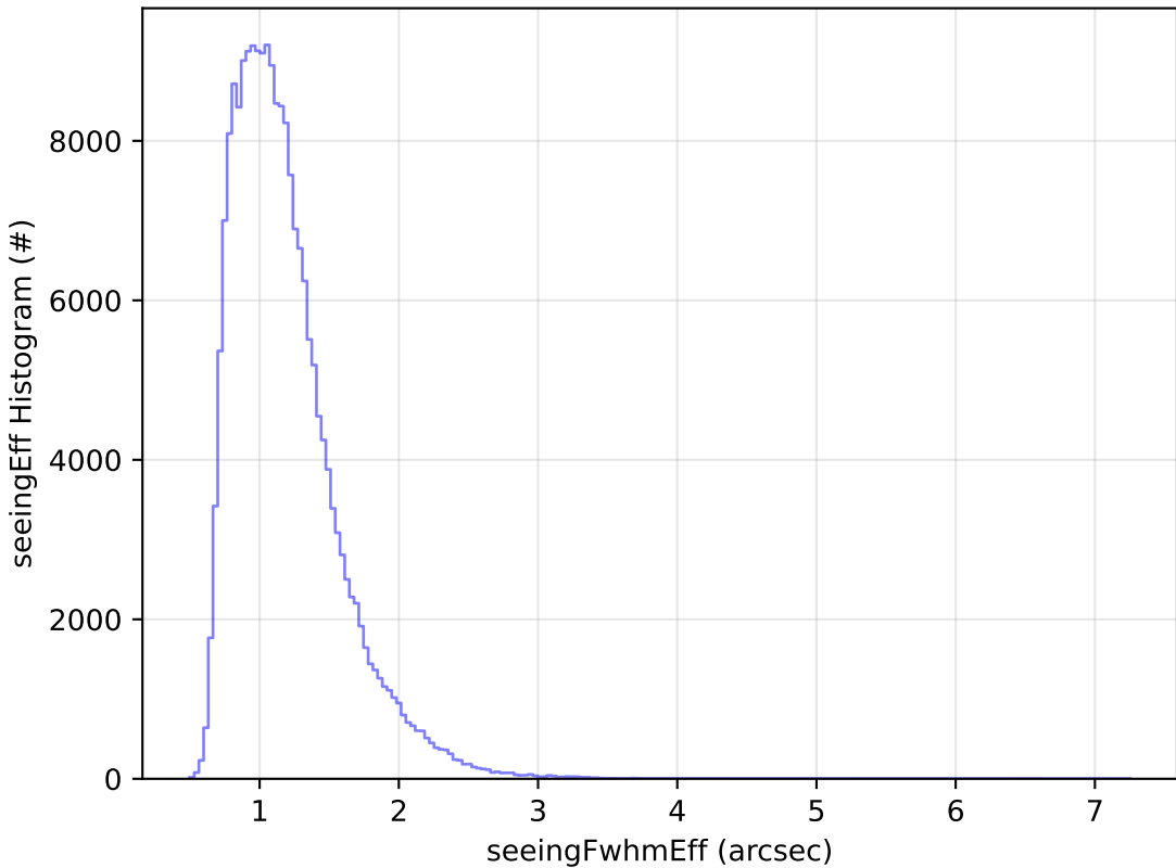
telescope_jerk_v3.5_10yrs WFD g band: seeingEff Histogram
