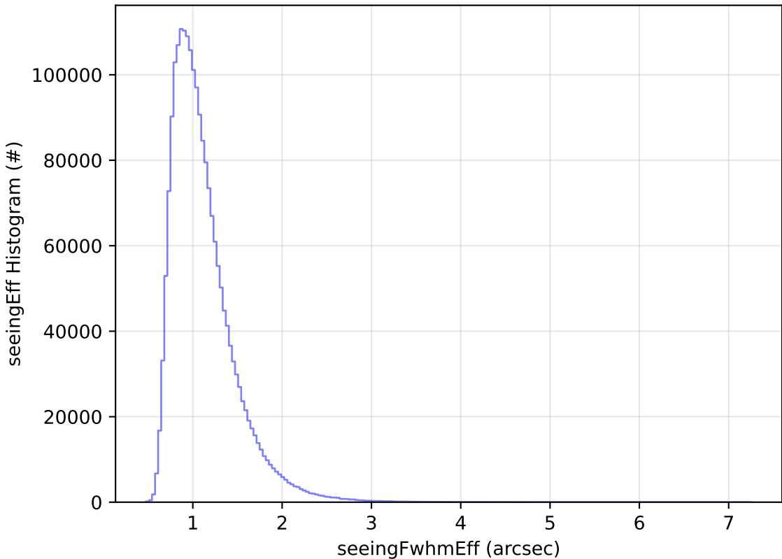
telescope_jerk_v3.5_10yrs WFD all bands: seeingEff Histogram
