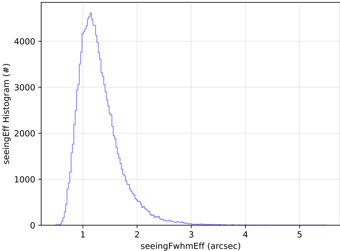
telescope_jerk_v3.5_10yrs All sky u band: seeingEff Histogram
