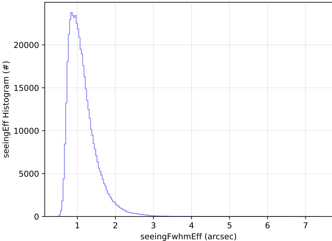
telescope_jerk_v3.5_10yrs All sky r band: seeingEff Histogram
