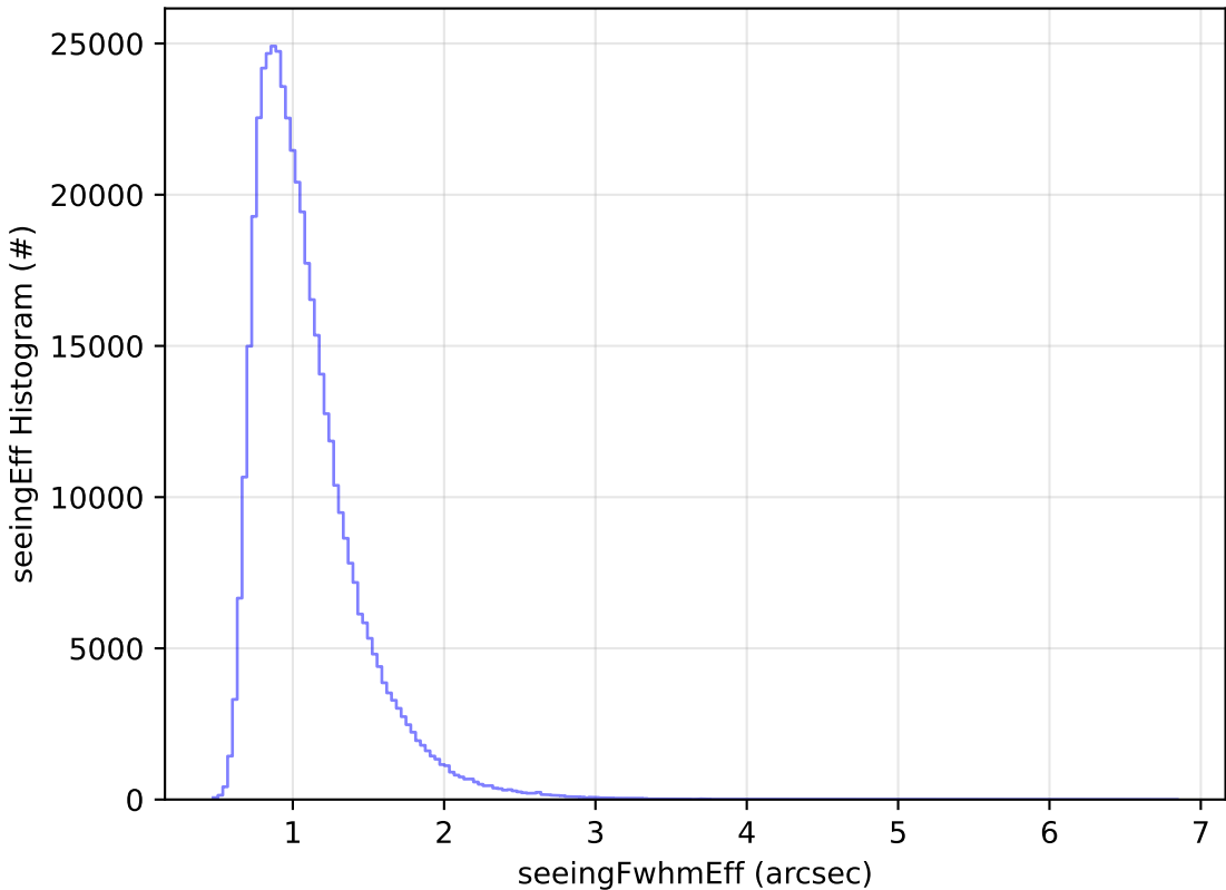
telescope_jerk_v3.5_10yrs All sky i band: seeingEff Histogram
