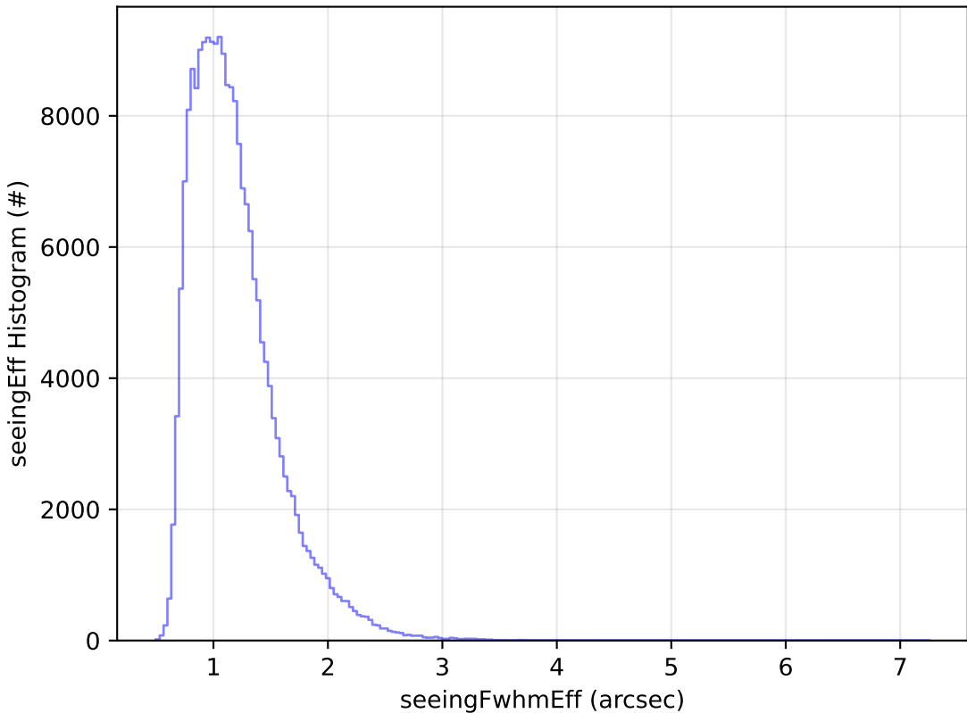
telescope_jerk_v3.5_10yrs All sky g band: seeingEff Histogram
