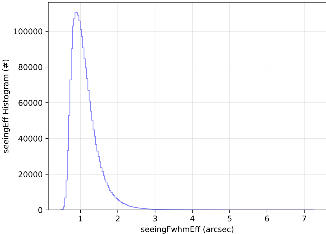
telescope_jerk_v3.5_10yrs All sky all bands: seeingEff Histogram
