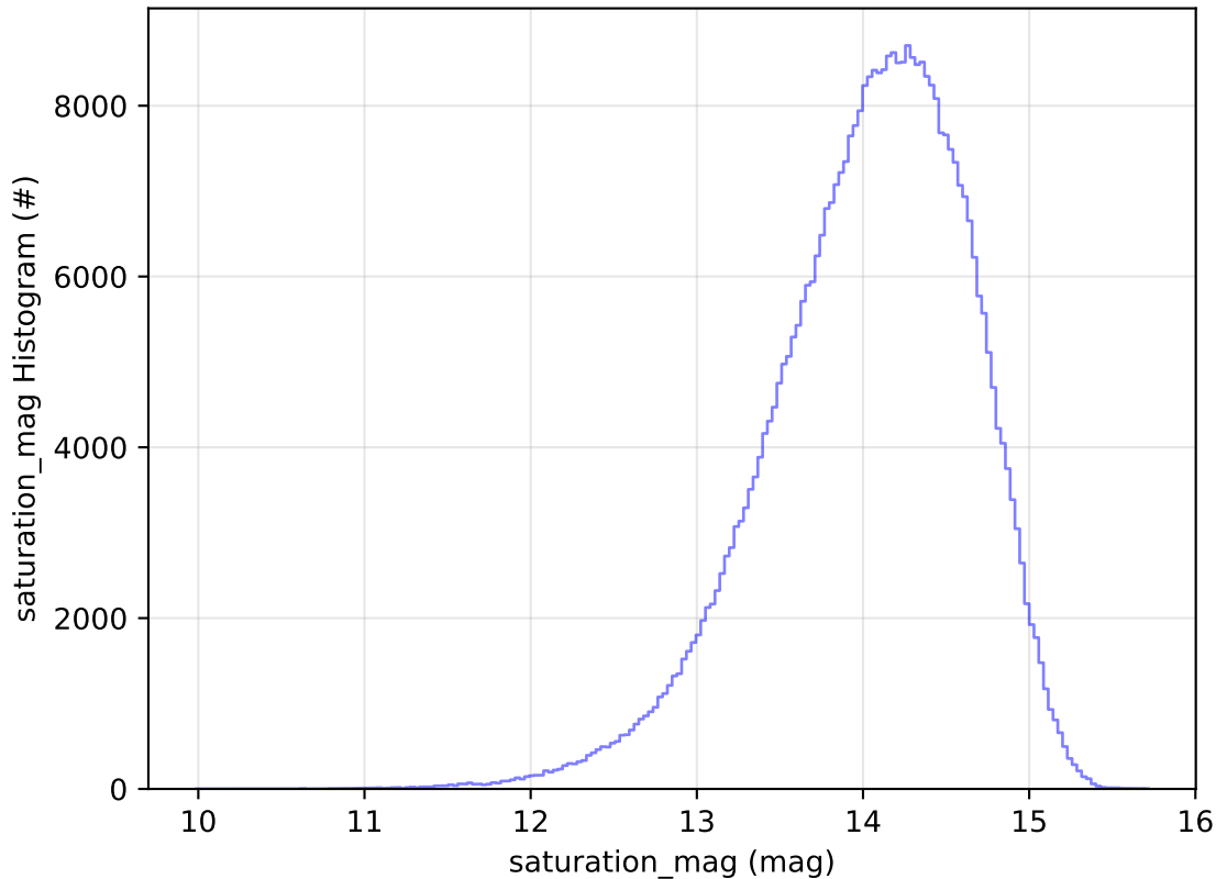
telescope_jerk_v3.5_10yrs WFD z band: saturation_mag Histogram
