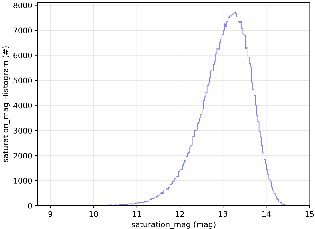
telescope_jerk_v3.5_10yrs WFD y band: saturation_mag Histogram
