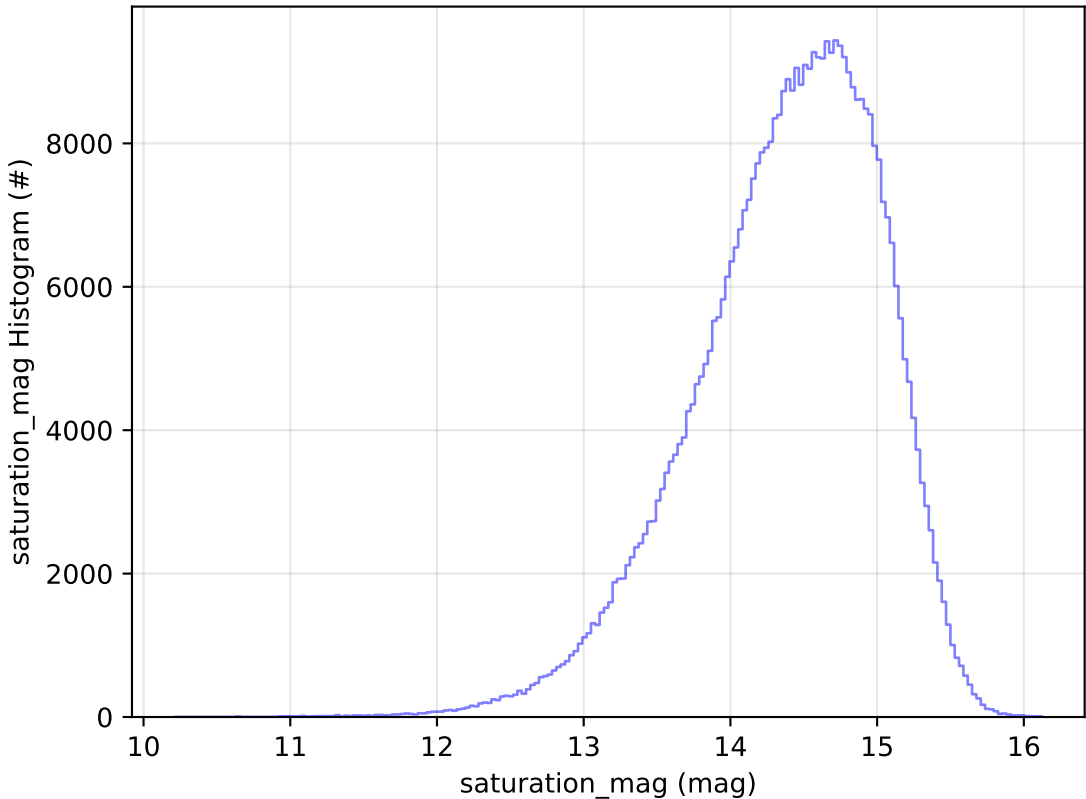
telescope_jerk_v3.5_10yrs WFD i band: saturation_mag Histogram
