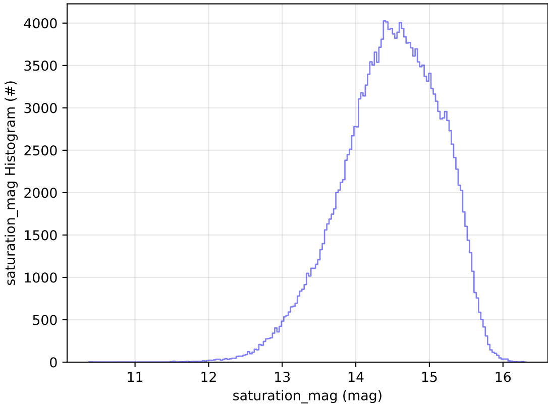
telescope_jerk_v3.5_10yrs WFD g band: saturation_mag Histogram
