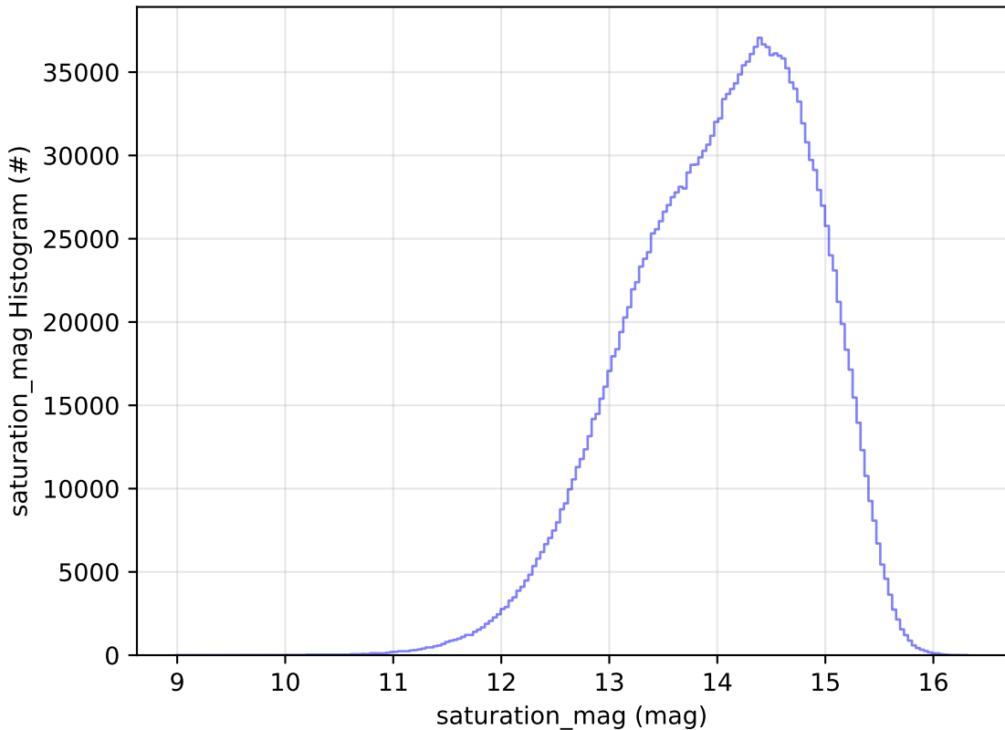
telescope_jerk_v3.5_10yrs WFD all bands: saturation_mag Histogram
