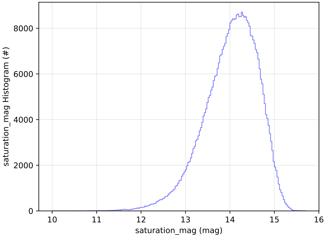
telescope_jerk_v3.5_10yrs All sky z band: saturation_mag Histogram
