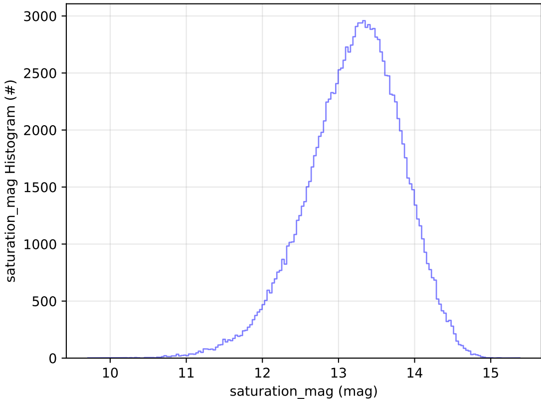
telescope_jerk_v3.5_10yrs All sky u band: saturation_mag Histogram
