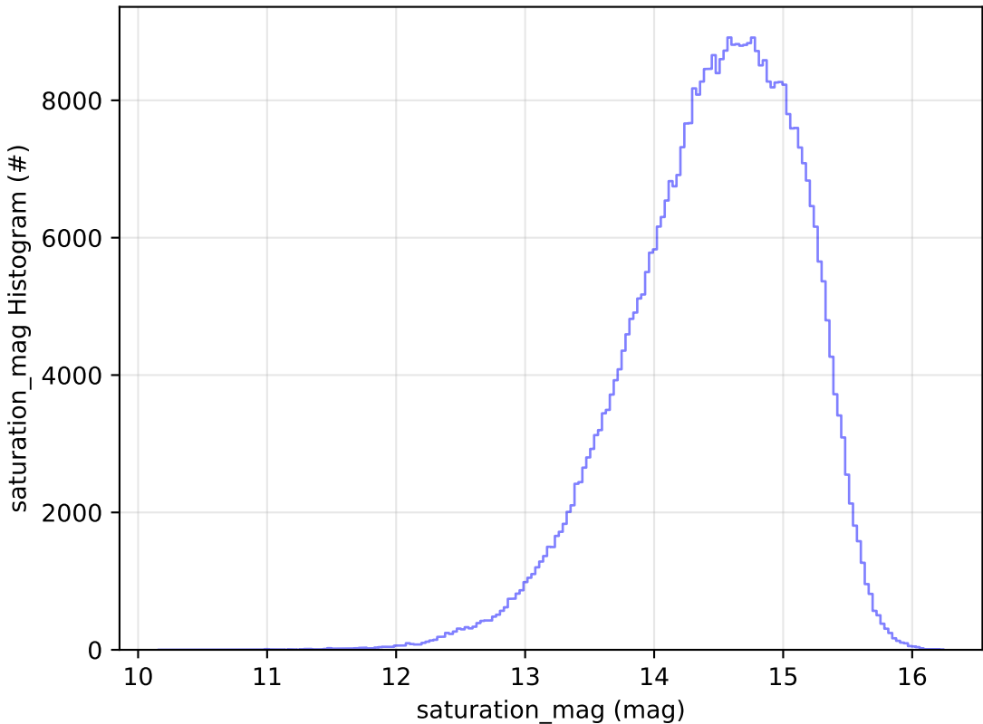
telescope_jerk_v3.5_10yrs All sky r band: saturation_mag Histogram
