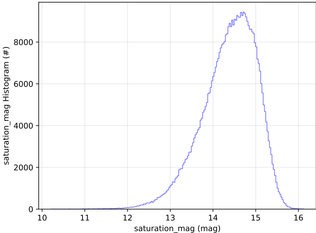
telescope_jerk_v3.5_10yrs All sky i band: saturation_mag Histogram
