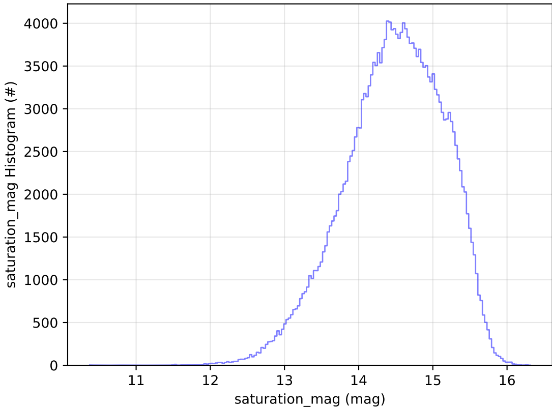
telescope_jerk_v3.5_10yrs All sky g band: saturation_mag Histogram
