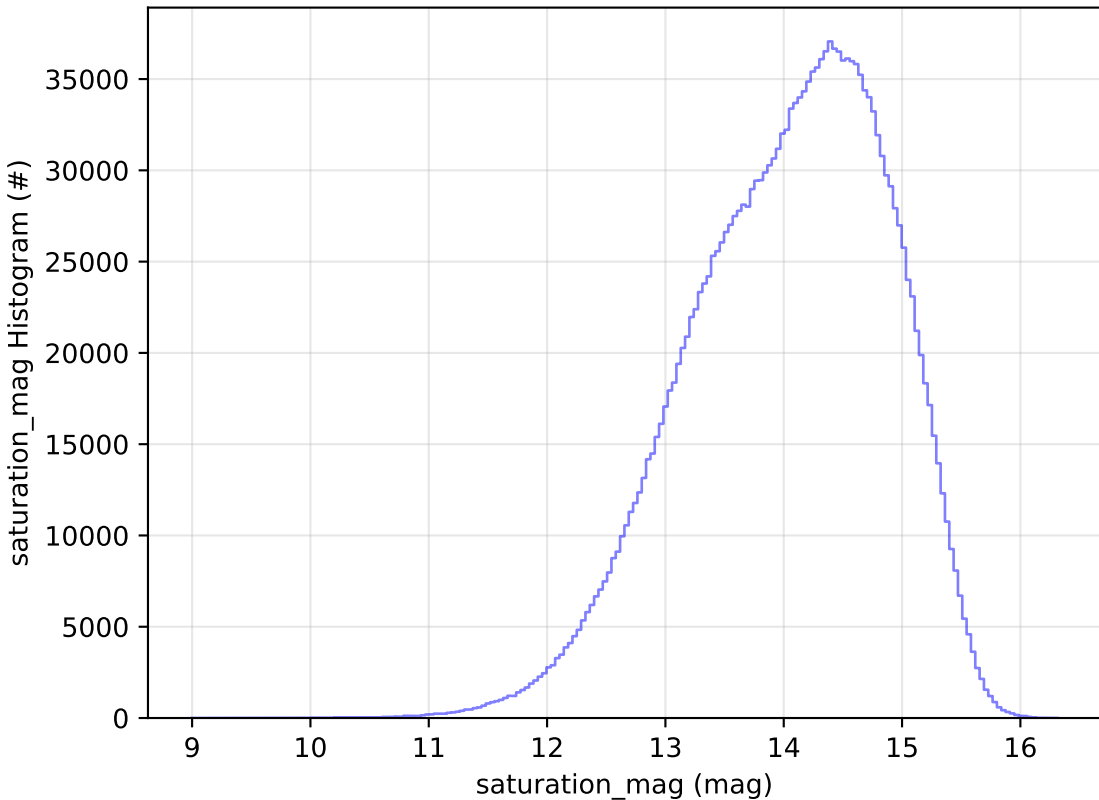
telescope_jerk_v3.5_10yrs All sky all bands: saturation_mag Histogram
