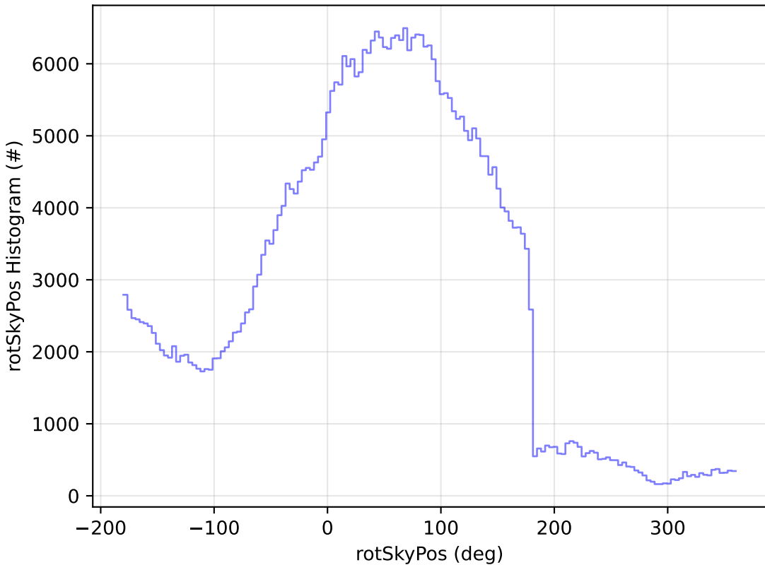
telescope_jerk_v3.5_10yrs WFD z band: rotSkyPos Histogram
