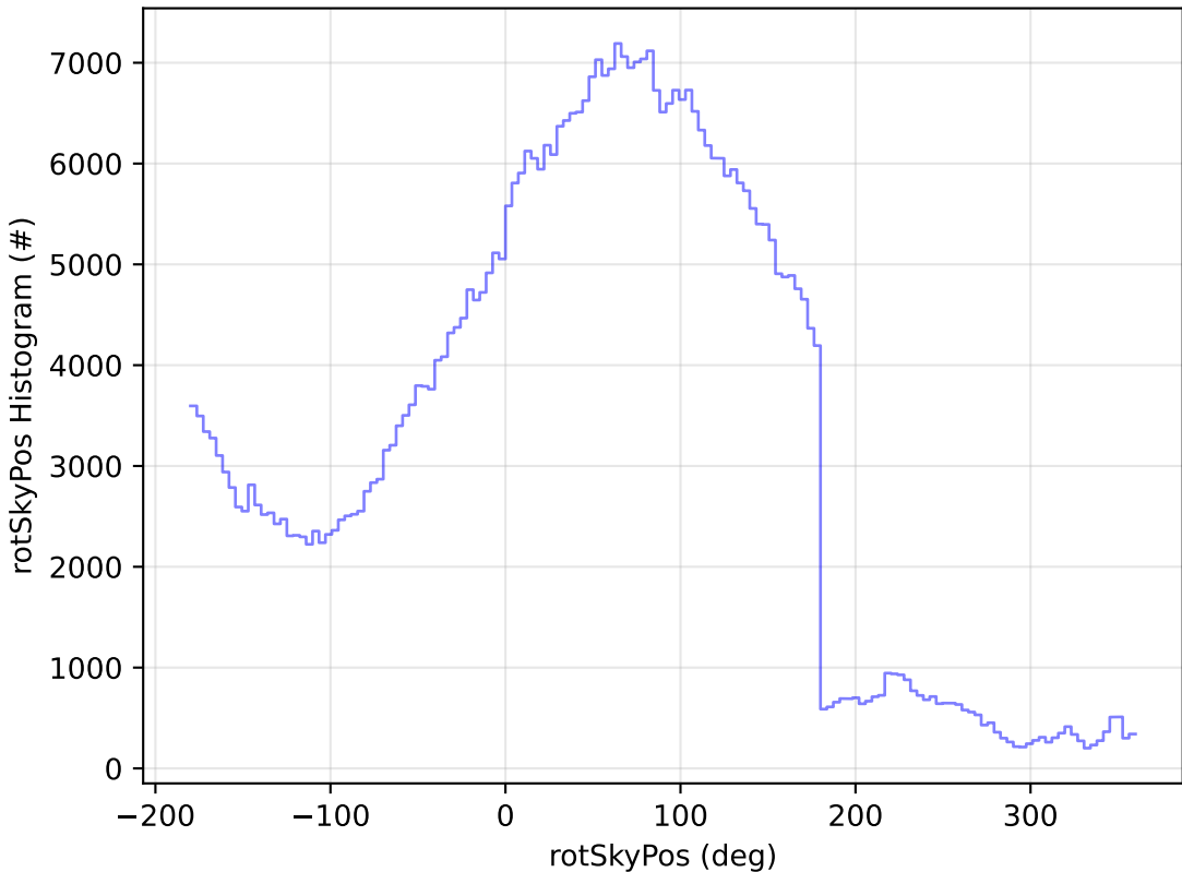
telescope_jerk_v3.5_10yrs WFD r band: rotSkyPos Histogram
