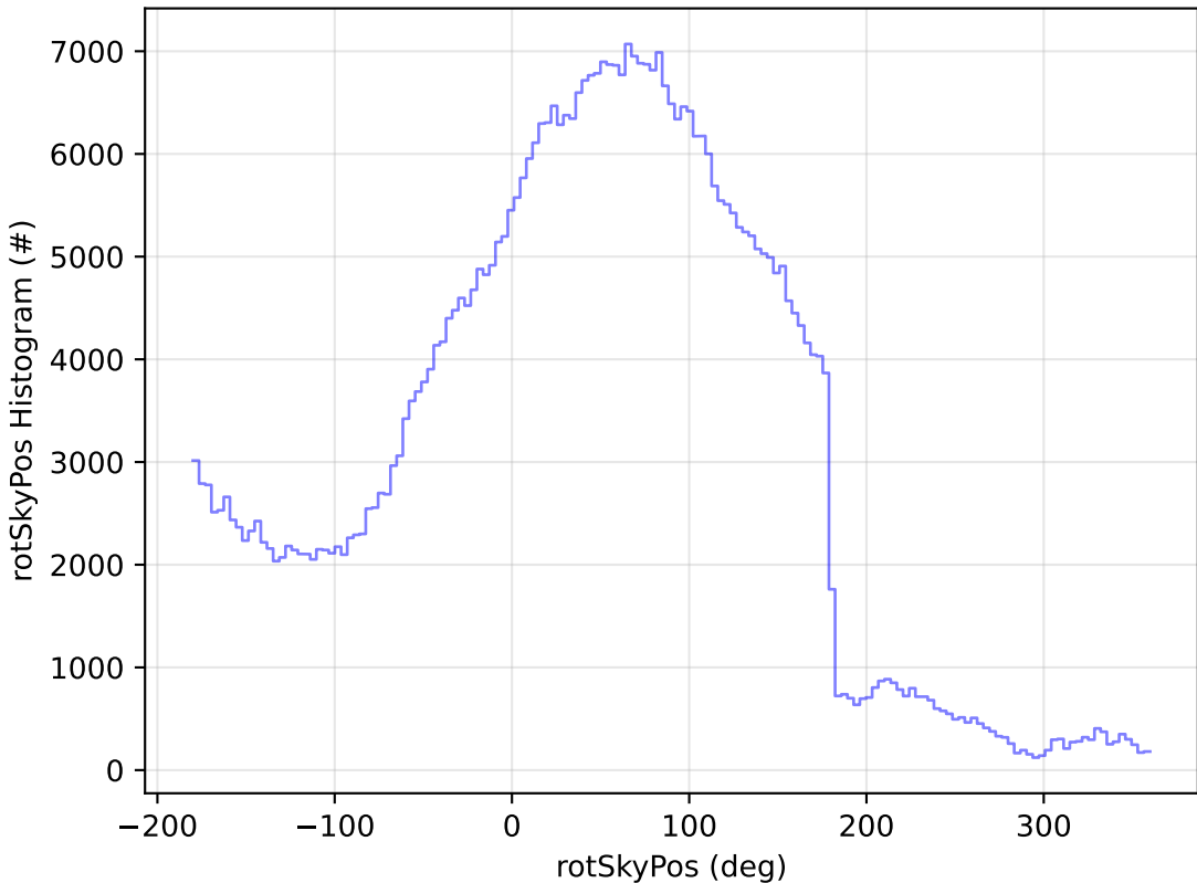
telescope_jerk_v3.5_10yrs WFD i band: rotSkyPos Histogram
