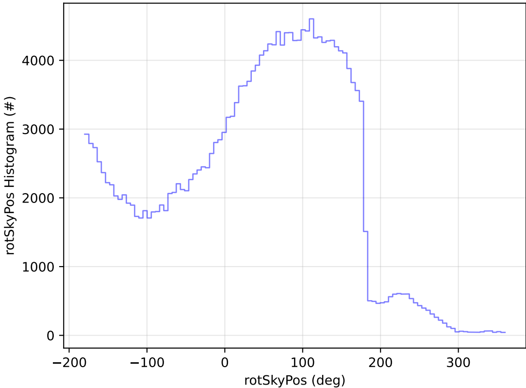
telescope_jerk_v3.5_10yrs WFD g band: rotSkyPos Histogram
