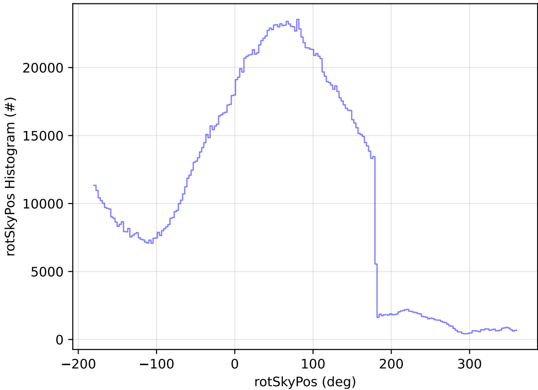
telescope_jerk_v3.5_10yrs WFD all bands: rotSkyPos Histogram
