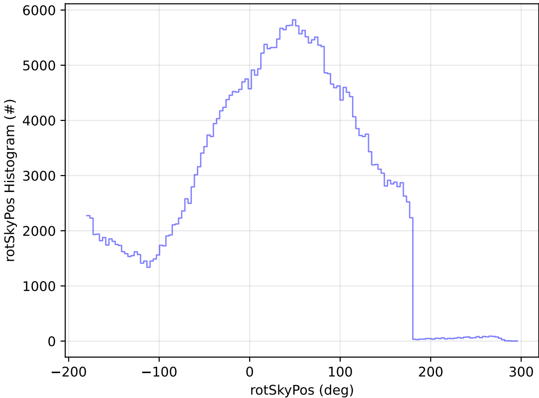
telescope_jerk_v3.5_10yrs All sky y band: rotSkyPos Histogram
