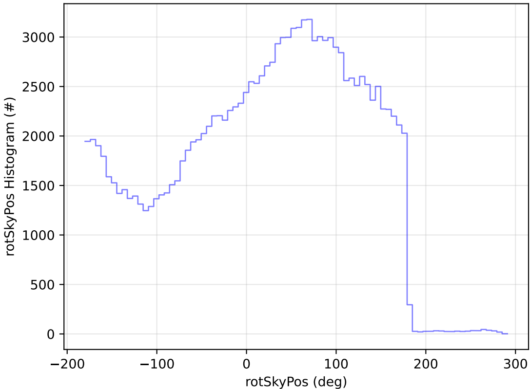
telescope_jerk_v3.5_10yrs All sky u band: rotSkyPos Histogram
