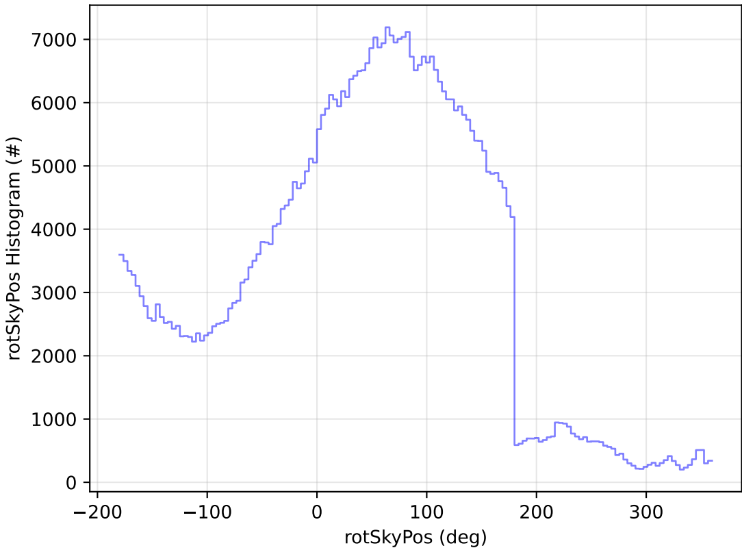
telescope_jerk_v3.5_10yrs All sky r band: rotSkyPos Histogram
