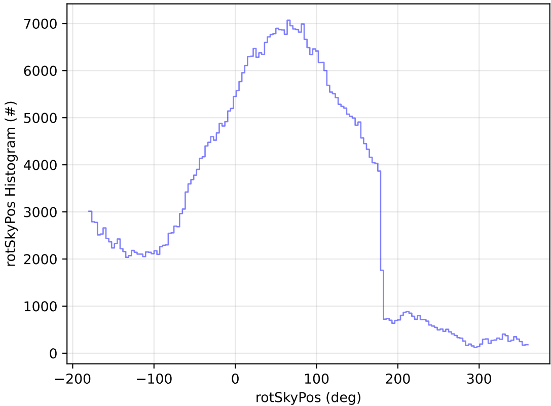
telescope_jerk_v3.5_10yrs All sky i band: rotSkyPos Histogram
